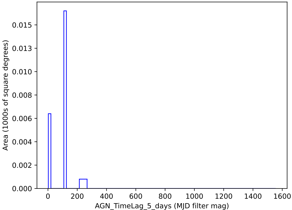
early_u_fpextra2.0_v3.4_10yrs y band: AGN_TimeLag_5_days
