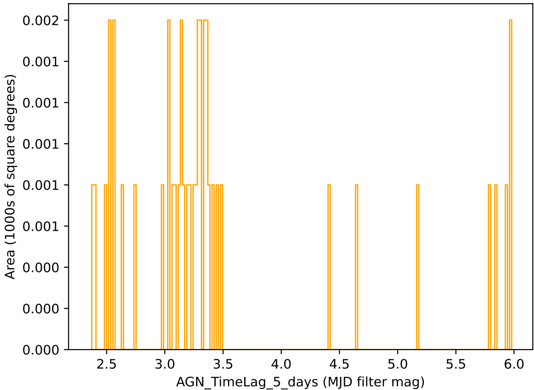
early_u_fpextra2.0_v3.4_10yrs r band: AGN_TimeLag_5_days
