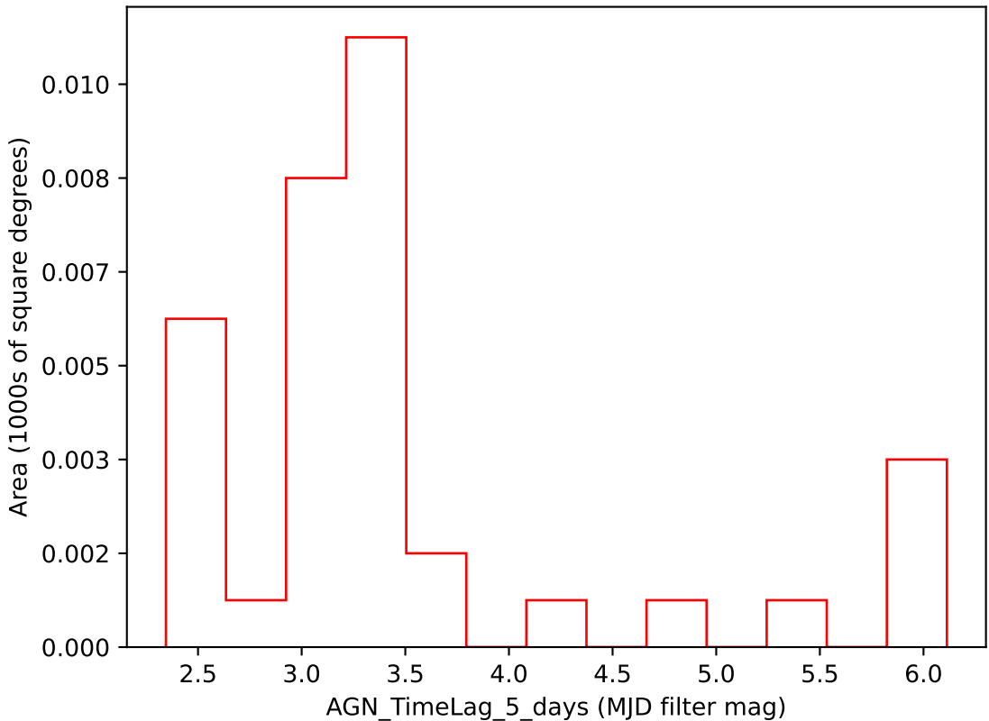
early_u_fpextra2.0_v3.4_10yrs i band: AGN_TimeLag_5_days
