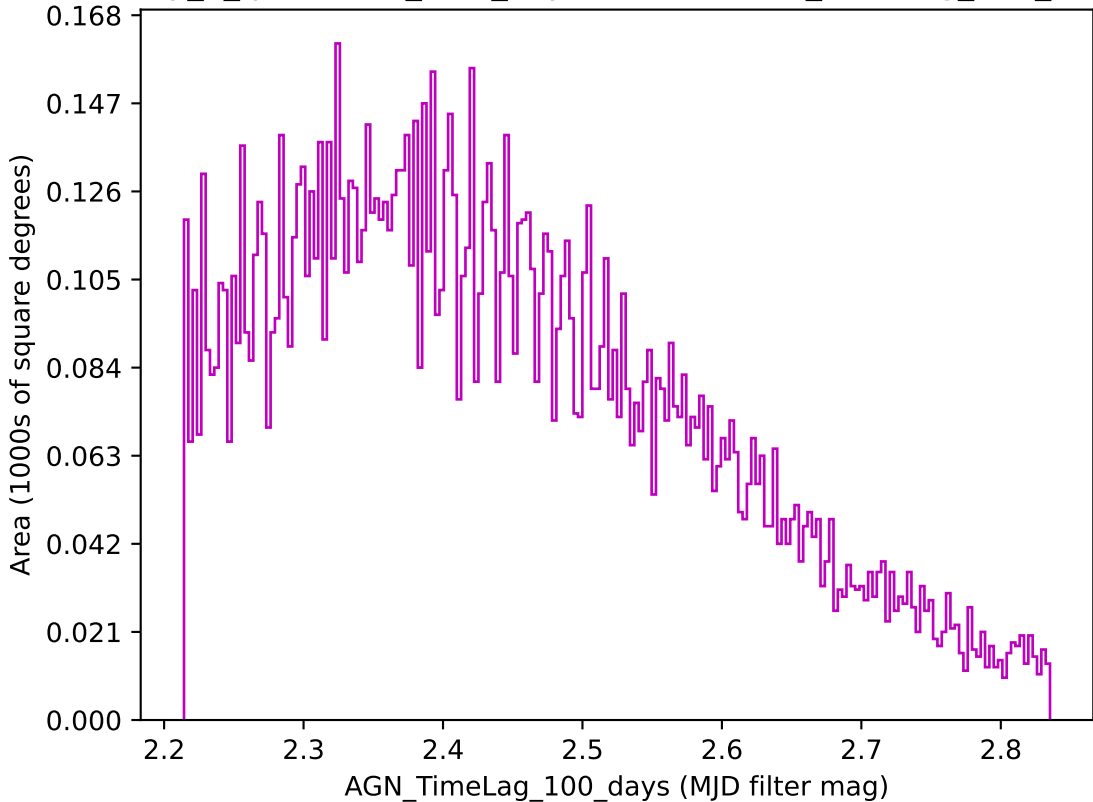
early_u_fpextra2.0_v3.4_10yrs z band: AGN_TimeLag_100_days
