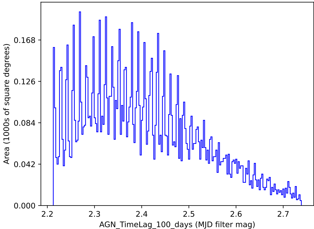
early_u_fpextra2.0_v3.4_10yrs y band: AGN_TimeLag_100_days
