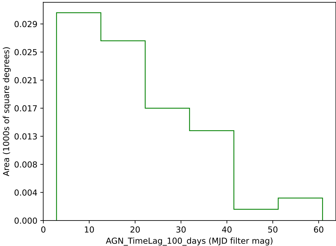
early_u_fpextra2.0_v3.4_10yrs g band: AGN_TimeLag_100_days
