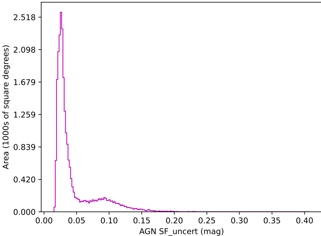
early_u_fpextra2.0_v3.4_10yrs z band: AGN SF_uncert
