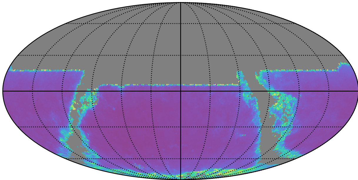
early_u_fpextra2.0_v3.4_10yrs y band: AGN SF_uncert
