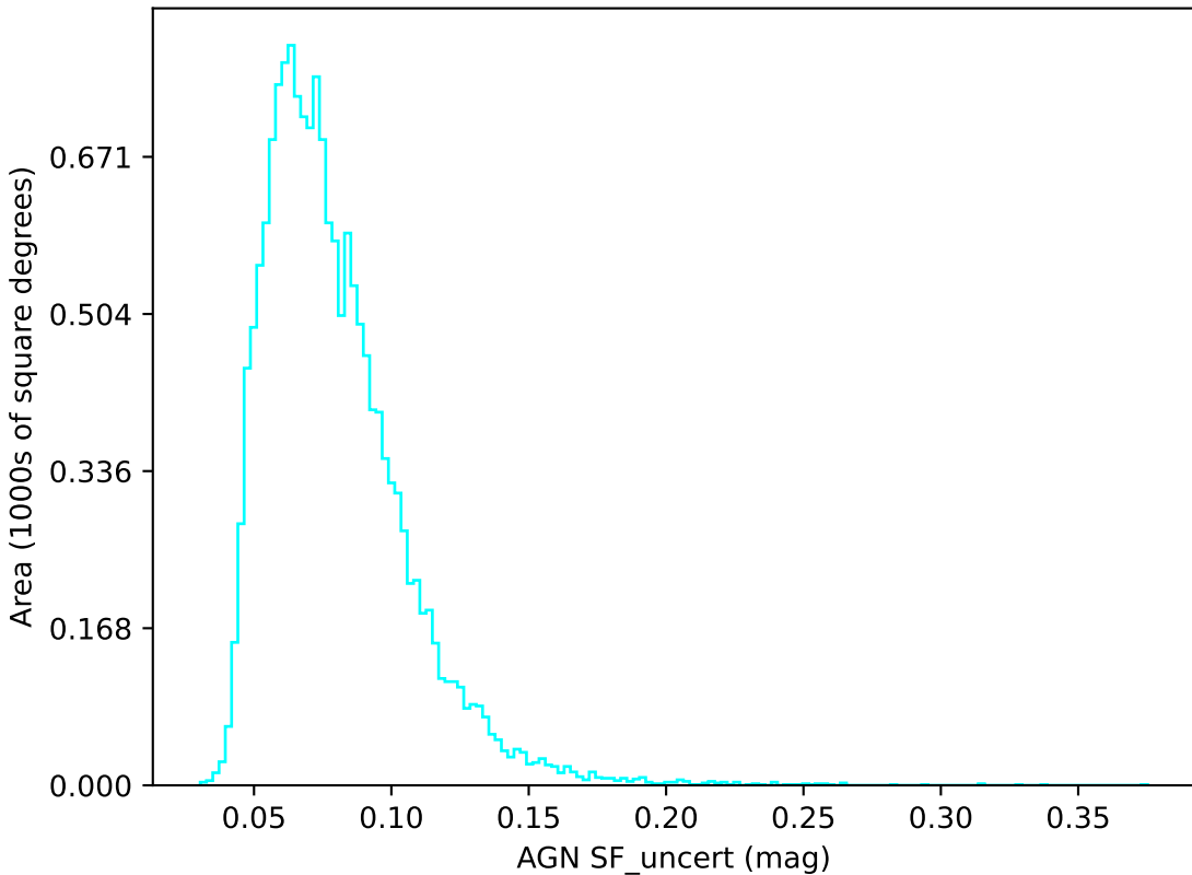
early_u_fpextra2.0_v3.4_10yrs u band: AGN SF_uncert
