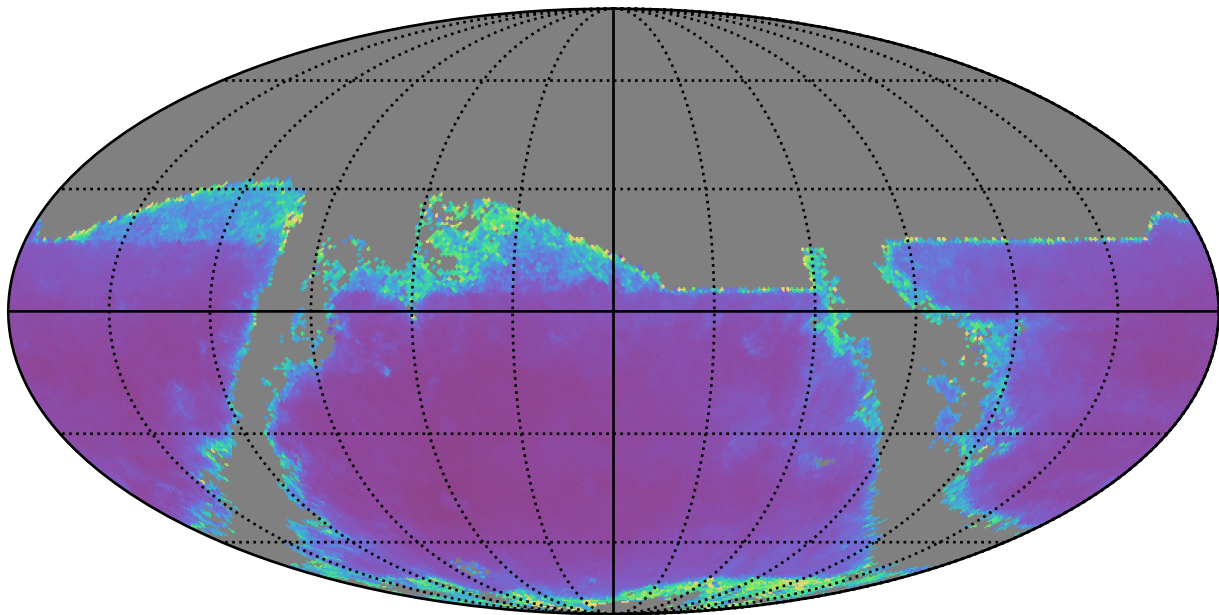
early_u_fpextra2.0_v3.4_10yrs r band: AGN SF_uncert
