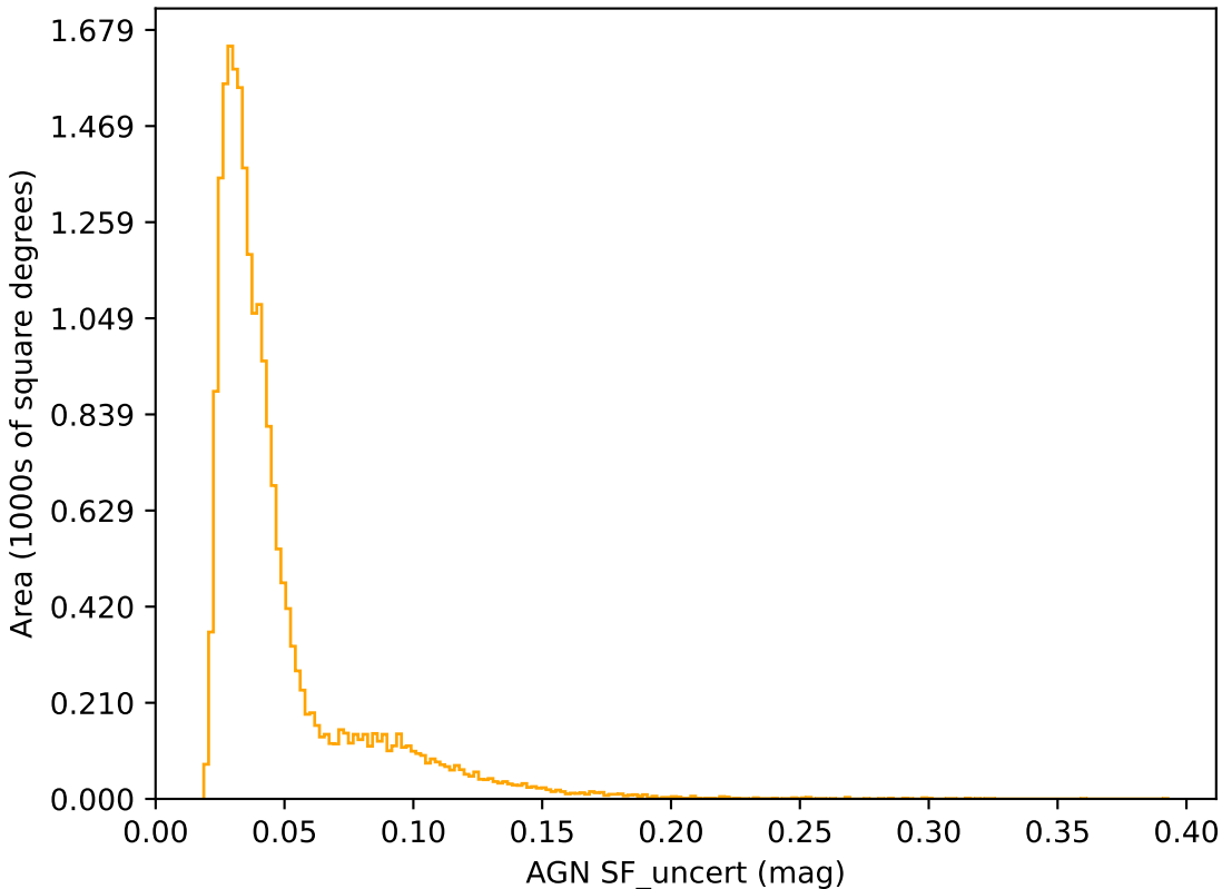
early_u_fpextra2.0_v3.4_10yrs r band: AGN SF_uncert
