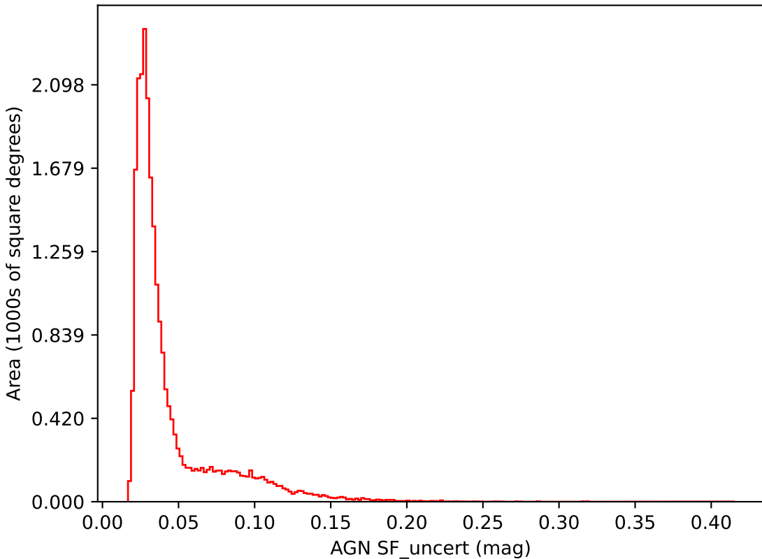
early_u_fpextra2.0_v3.4_10yrs i band: AGN SF_uncert
