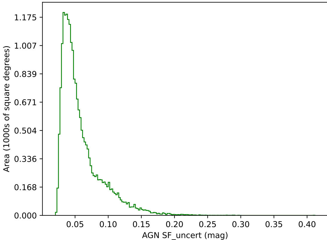
early_u_fpextra2.0_v3.4_10yrs g band: AGN SF_uncert
