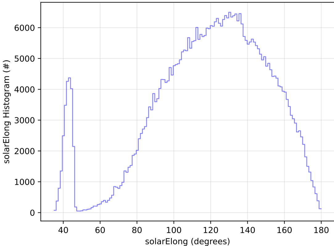
early_u_fpextra2.0_v3.4_10yrs WFD z band: solarElong Histogram
