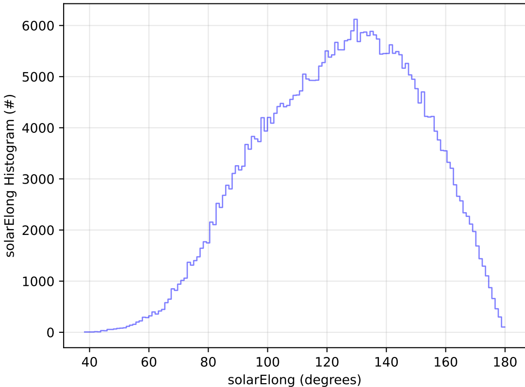
early_u_fpextra2.0_v3.4_10yrs WFD y band: solarElong Histogram
