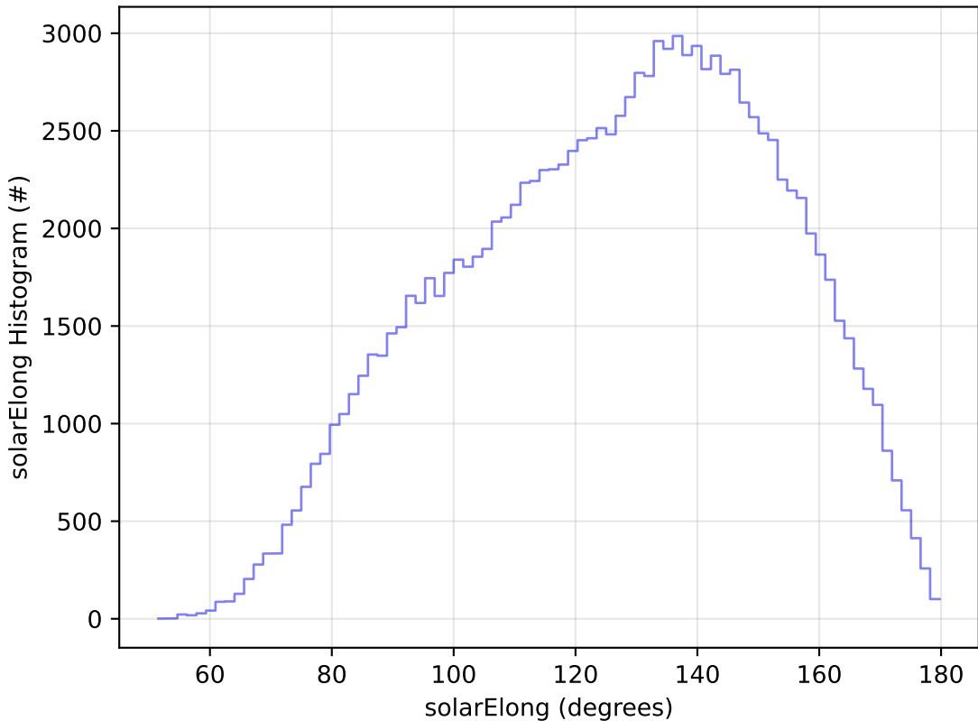
early_u_fpextra2.0_v3.4_10yrs WFD u band: solarElong Histogram
