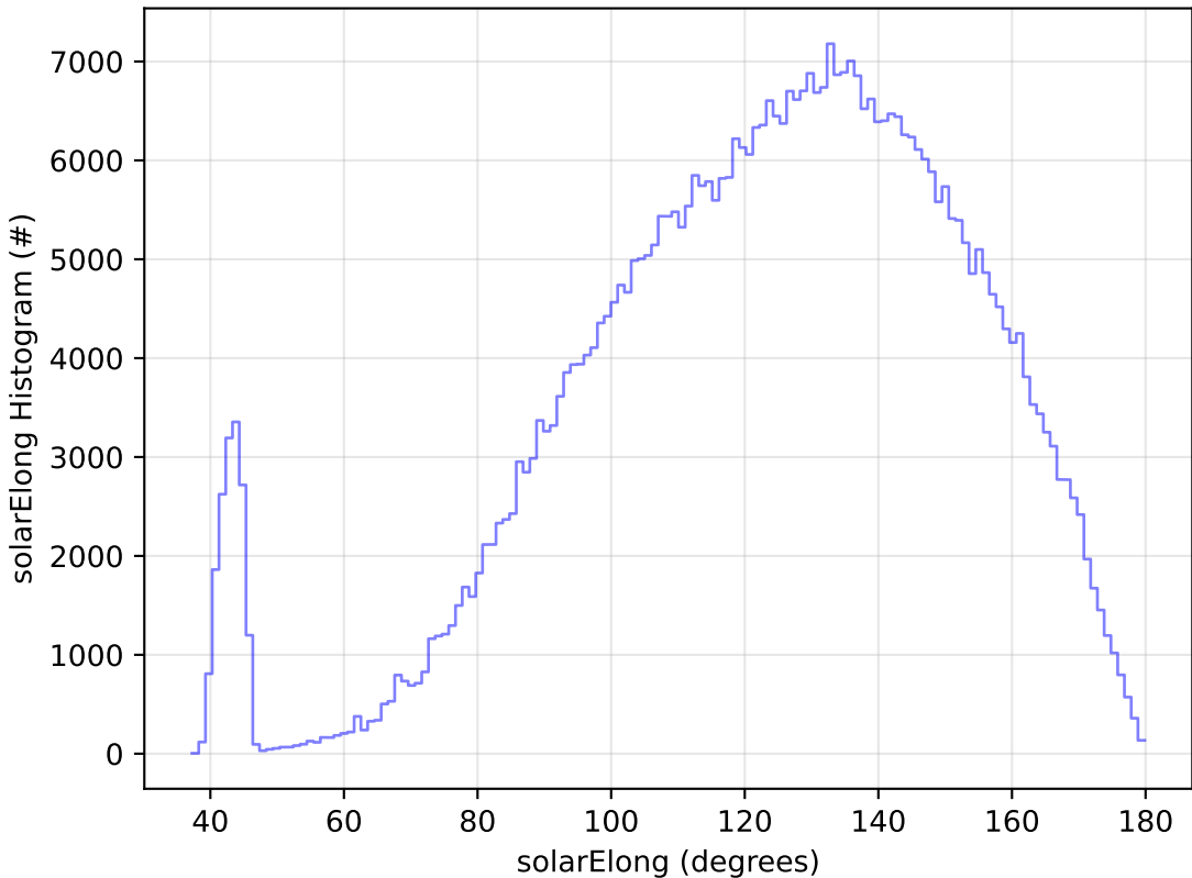
early_u_fpextra2.0_v3.4_10yrs WFD r band: solarElong Histogram
