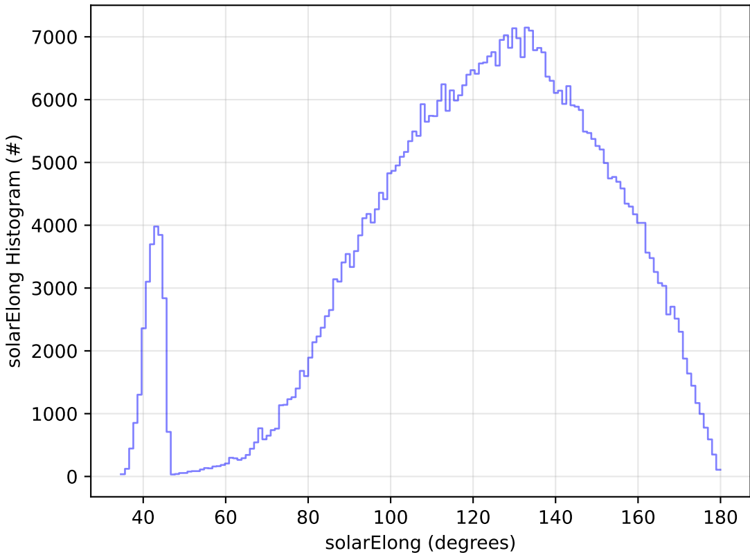
early_u_fpextra2.0_v3.4_10yrs WFD i band: solarElong Histogram
