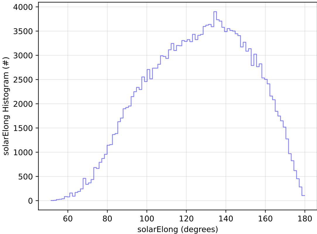
early_u_fpextra2.0_v3.4_10yrs WFD g band: solarElong Histogram
