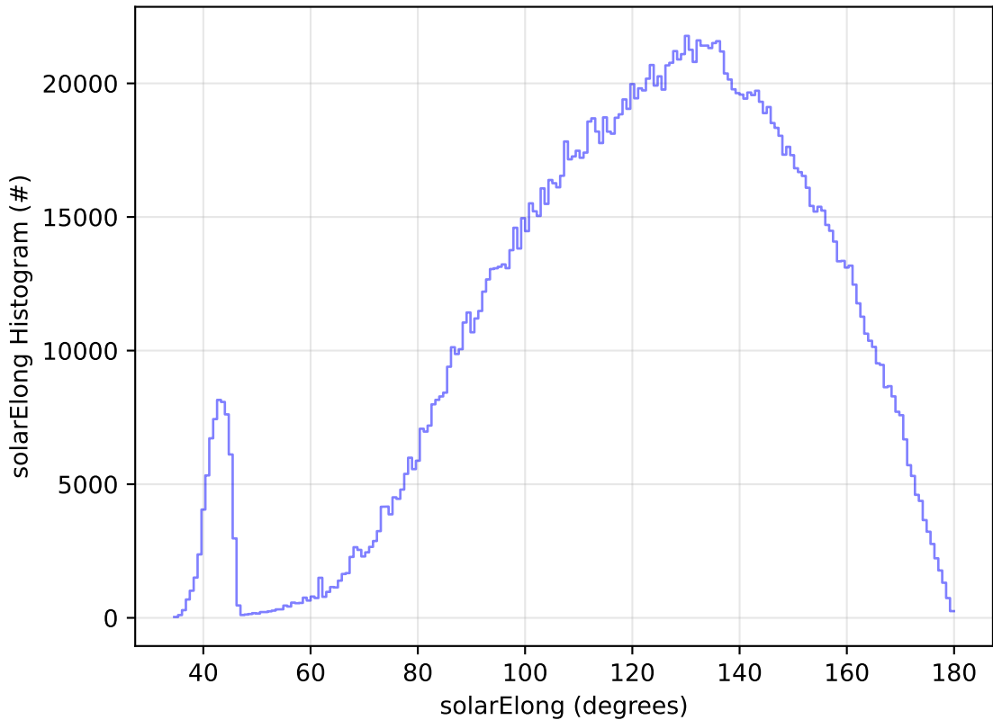
early_u_fpextra2.0_v3.4_10yrs WFD all bands: solarElong Histogram
