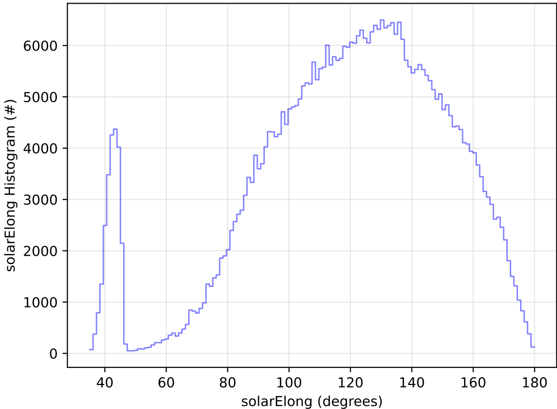
early_u_fpextra2.0_v3.4_10yrs All sky z band: solarElong Histogram
