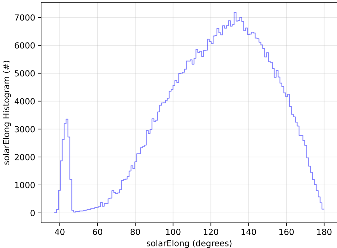
early_u_fpextra2.0_v3.4_10yrs All sky r band: solarElong Histogram
