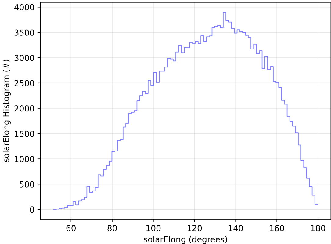
early_u_fpextra2.0_v3.4_10yrs All sky g band: solarElong Histogram
