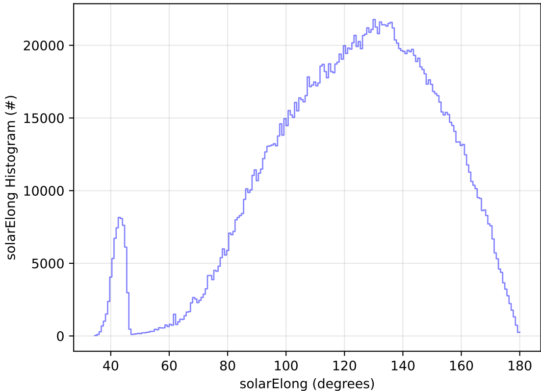
early_u_fpextra2.0_v3.4_10yrs All sky all bands: solarElong Histogram
