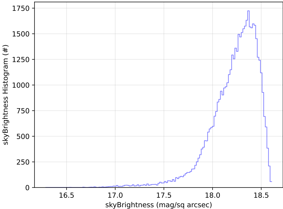
early_u_fpextra2.0_v3.4_10yrs Yr 1 y band: skyBrightness Histogram
