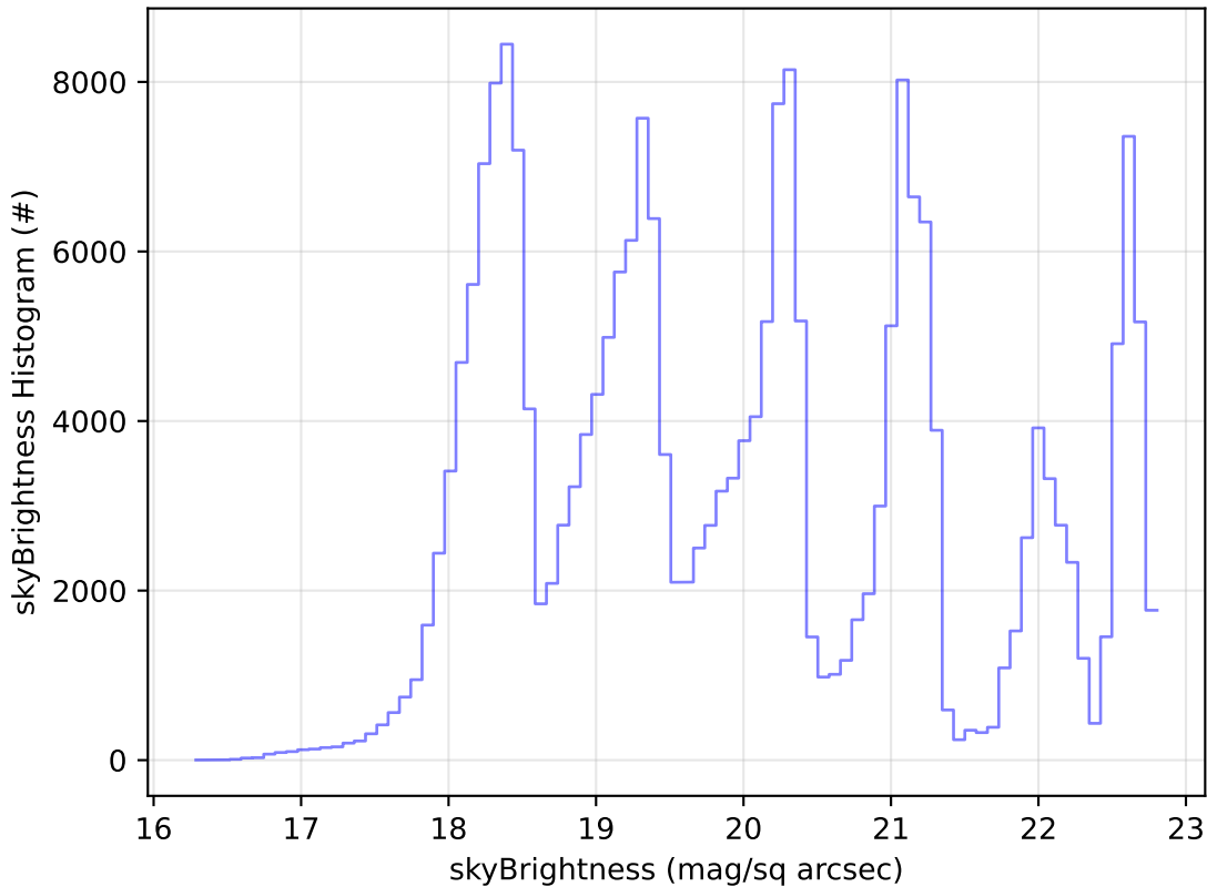
early_u_fpextra2.0_v3.4_10yrs Yr 1 all bands: skyBrightness Histogram
