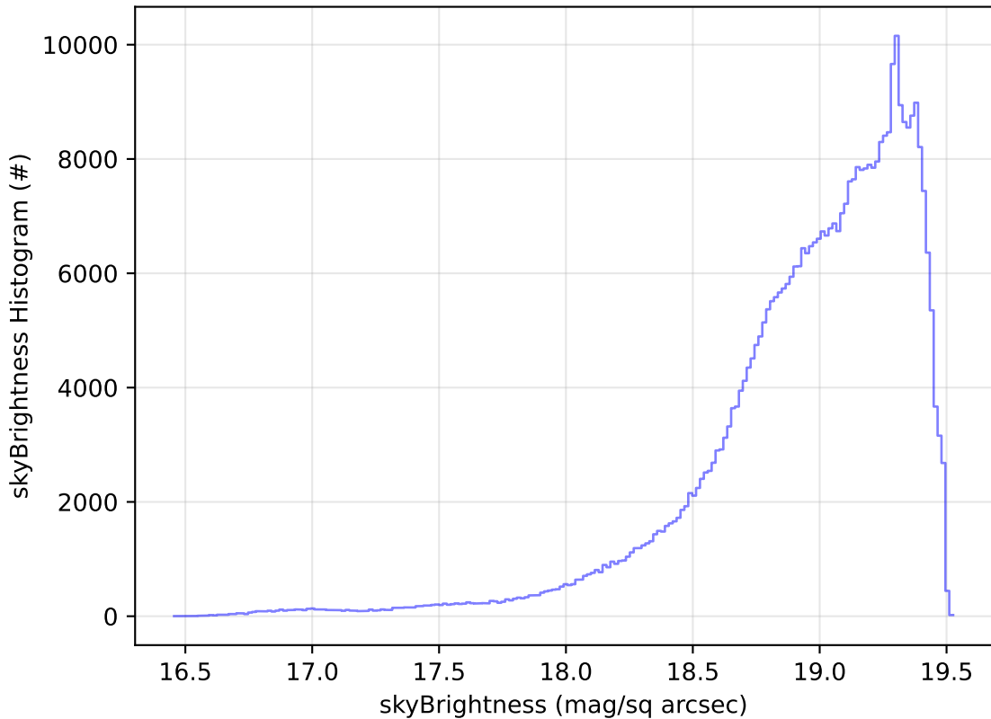
early_u_fpextra2.0_v3.4_10yrs WFD z band: skyBrightness Histogram
