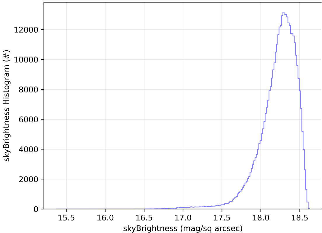
early_u_fpextra2.0_v3.4_10yrs WFD y band: skyBrightness Histogram
