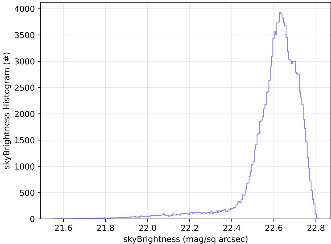
early_u_fpextra2.0_v3.4_10yrs WFD u band: skyBrightness Histogram
