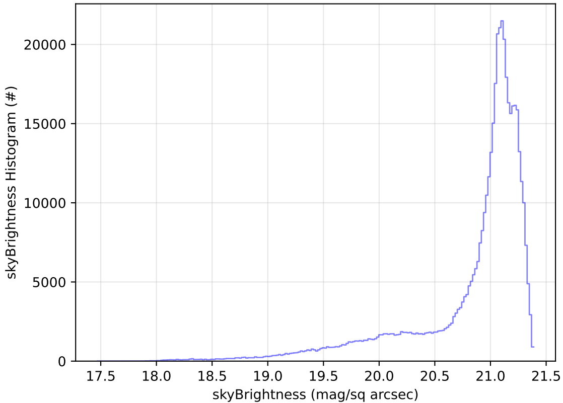
early_u_fpextra2.0_v3.4_10yrs WFD r band: skyBrightness Histogram
