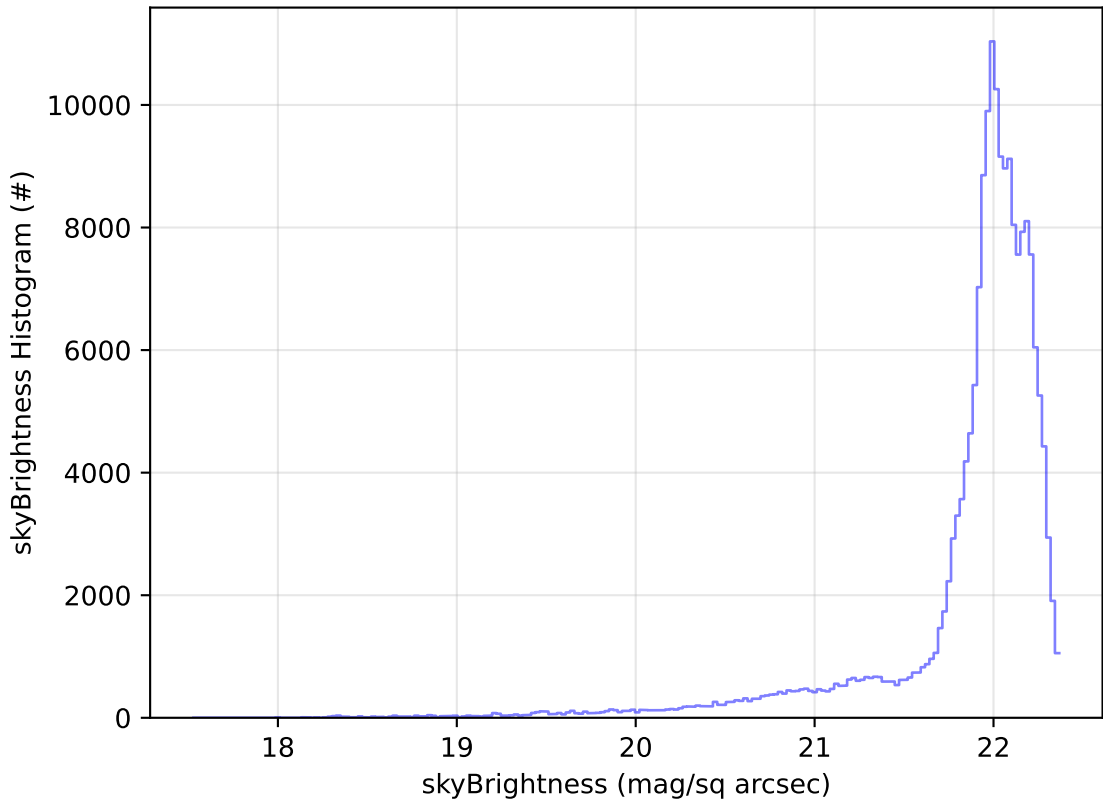
early_u_fpextra2.0_v3.4_10yrs WFD g band: skyBrightness Histogram
