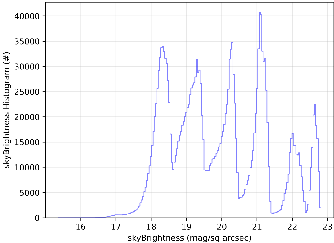
early_u_fpextra2.0_v3.4_10yrs WFD all bands: skyBrightness Histogram
