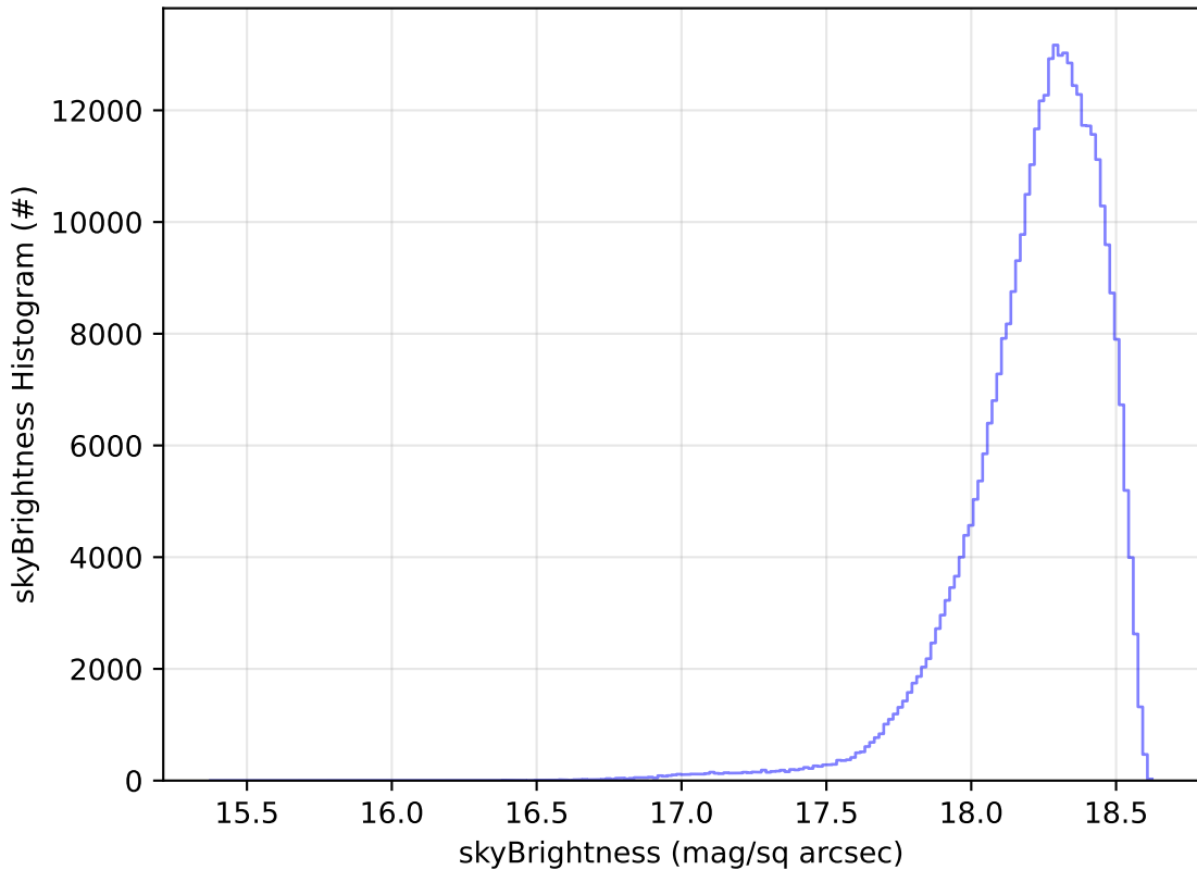
early_u_fpextra2.0_v3.4_10yrs All sky y band: skyBrightness Histogram
