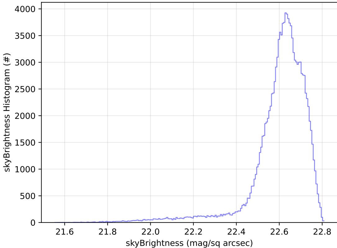
early_u_fpextra2.0_v3.4_10yrs All sky u band: skyBrightness Histogram
