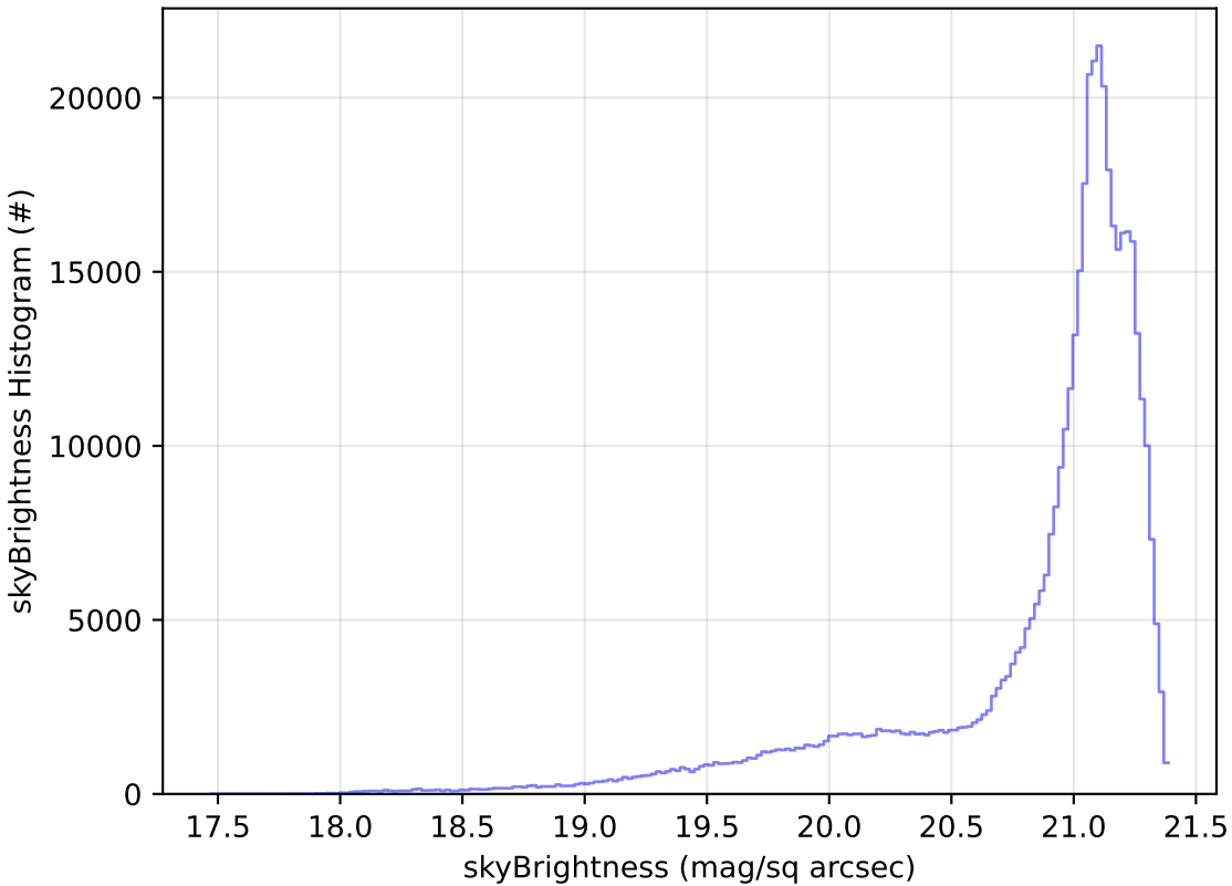
early_u_fpextra2.0_v3.4_10yrs All sky r band: skyBrightness Histogram
