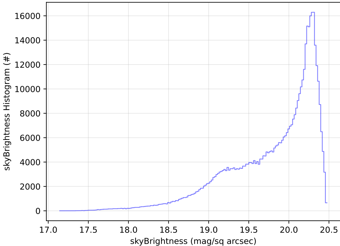
early_u_fpextra2.0_v3.4_10yrs All sky i band: skyBrightness Histogram
