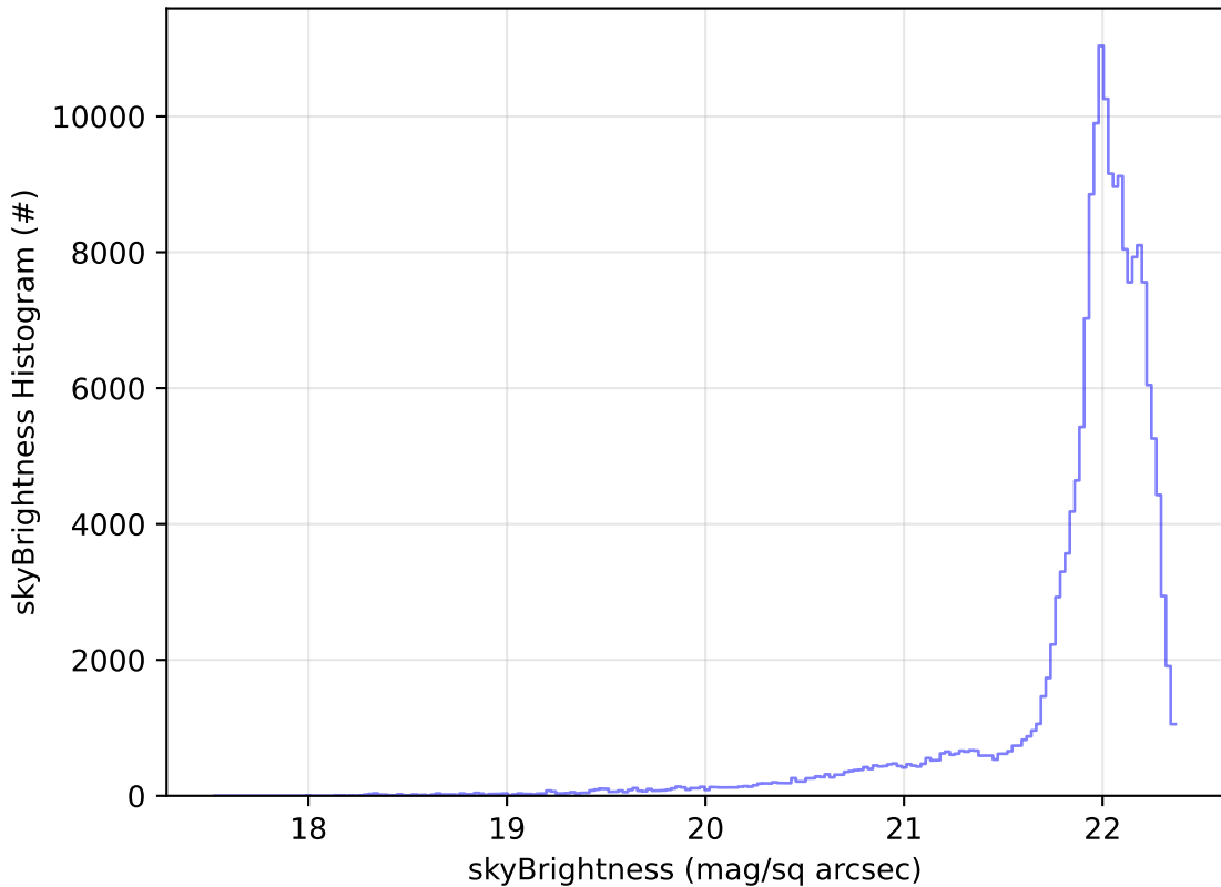
early_u_fpextra2.0_v3.4_10yrs All sky g band: skyBrightness Histogram
