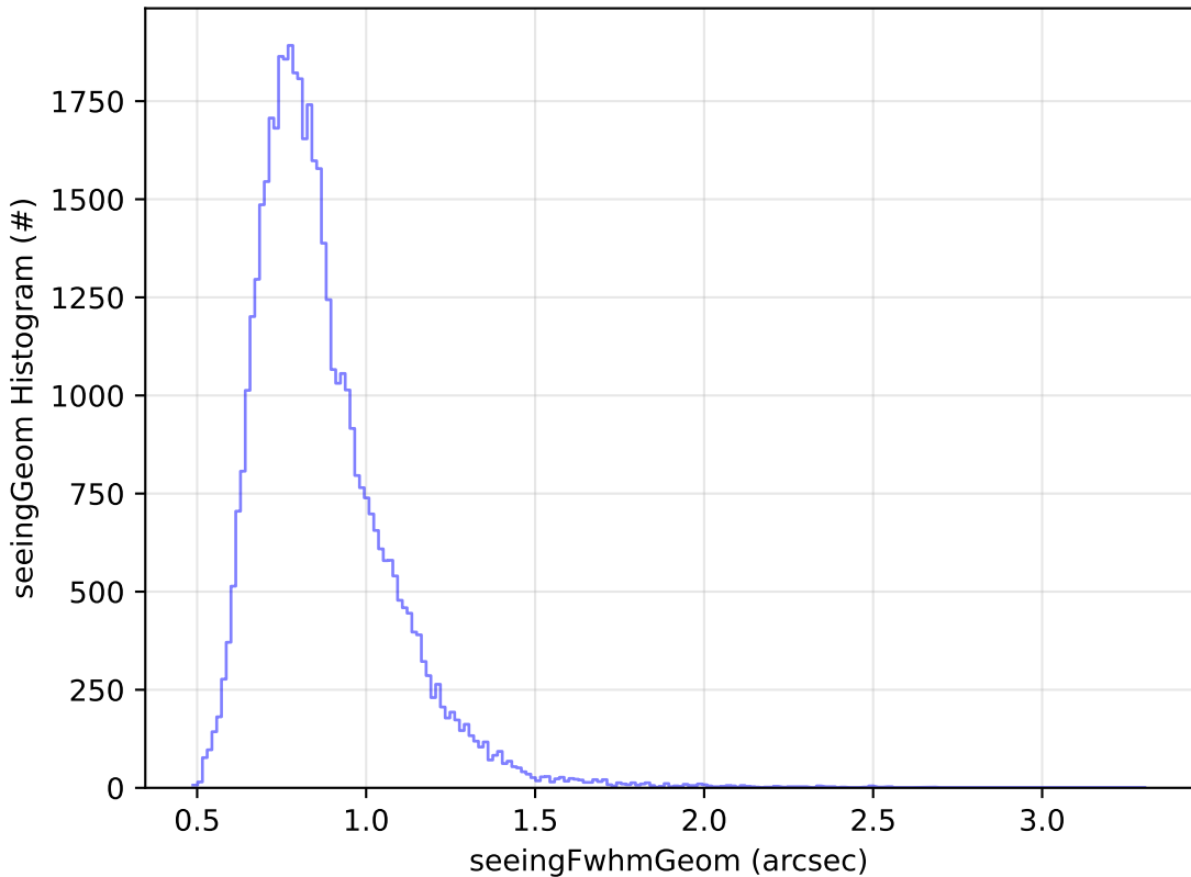
early_u_fpextra2.0_v3.4_10yrs Yr 1 y band: seeingGeom Histogram
