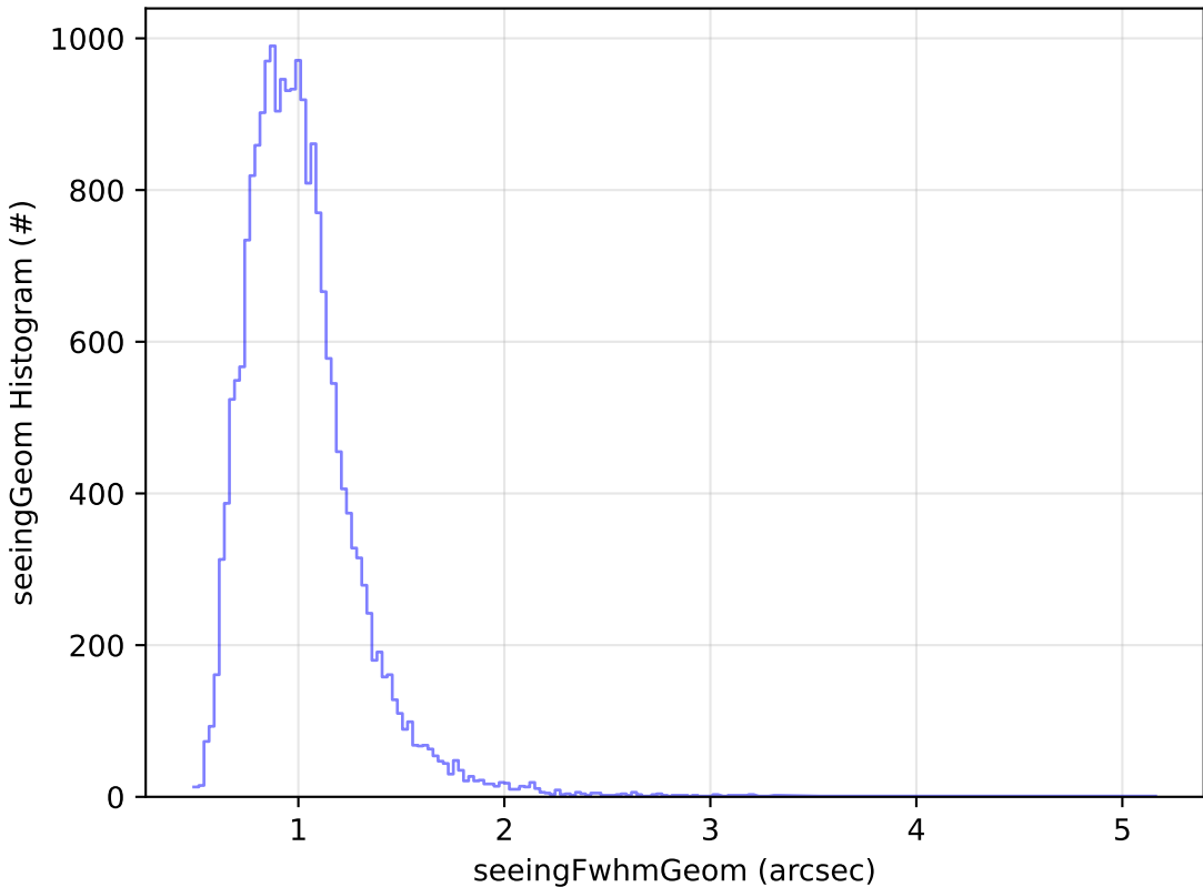
early_u_fpextra2.0_v3.4_10yrs Yr 1 u band: seeingGeom Histogram
