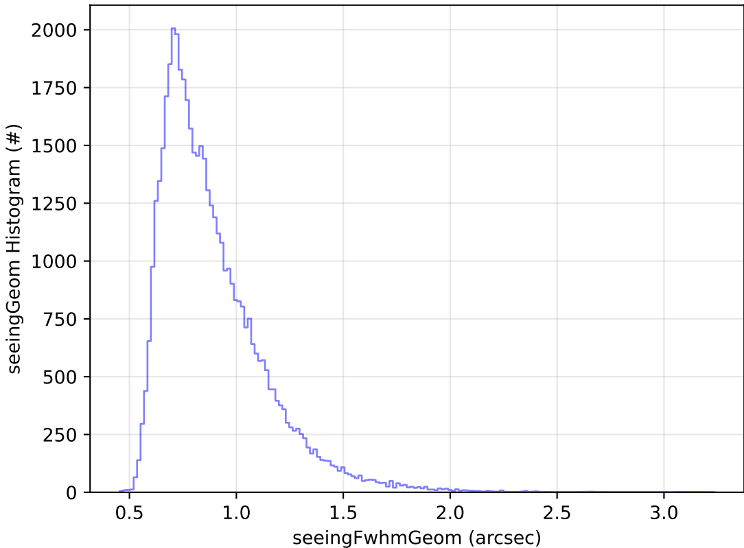
early_u_fpextra2.0_v3.4_10yrs Yr 1 r band: seeingGeom Histogram
