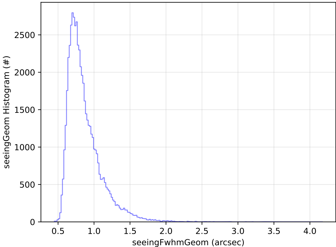
early_u_fpextra2.0_v3.4_10yrs Yr 1 i band: seeingGeom Histogram
