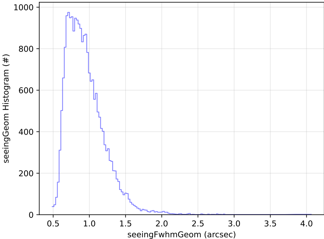
early_u_fpextra2.0_v3.4_10yrs Yr 1 g band: seeingGeom Histogram
