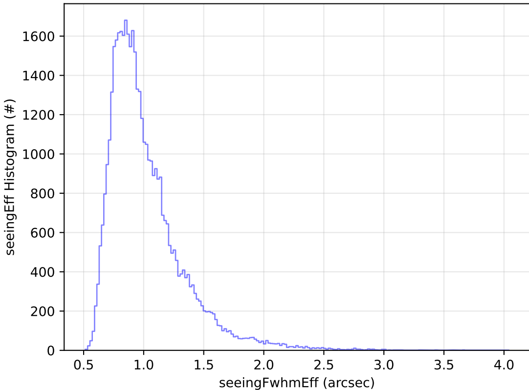
early_u_fpextra2.0_v3.4_10yrs Yr 1 z band: seeingEff Histogram
