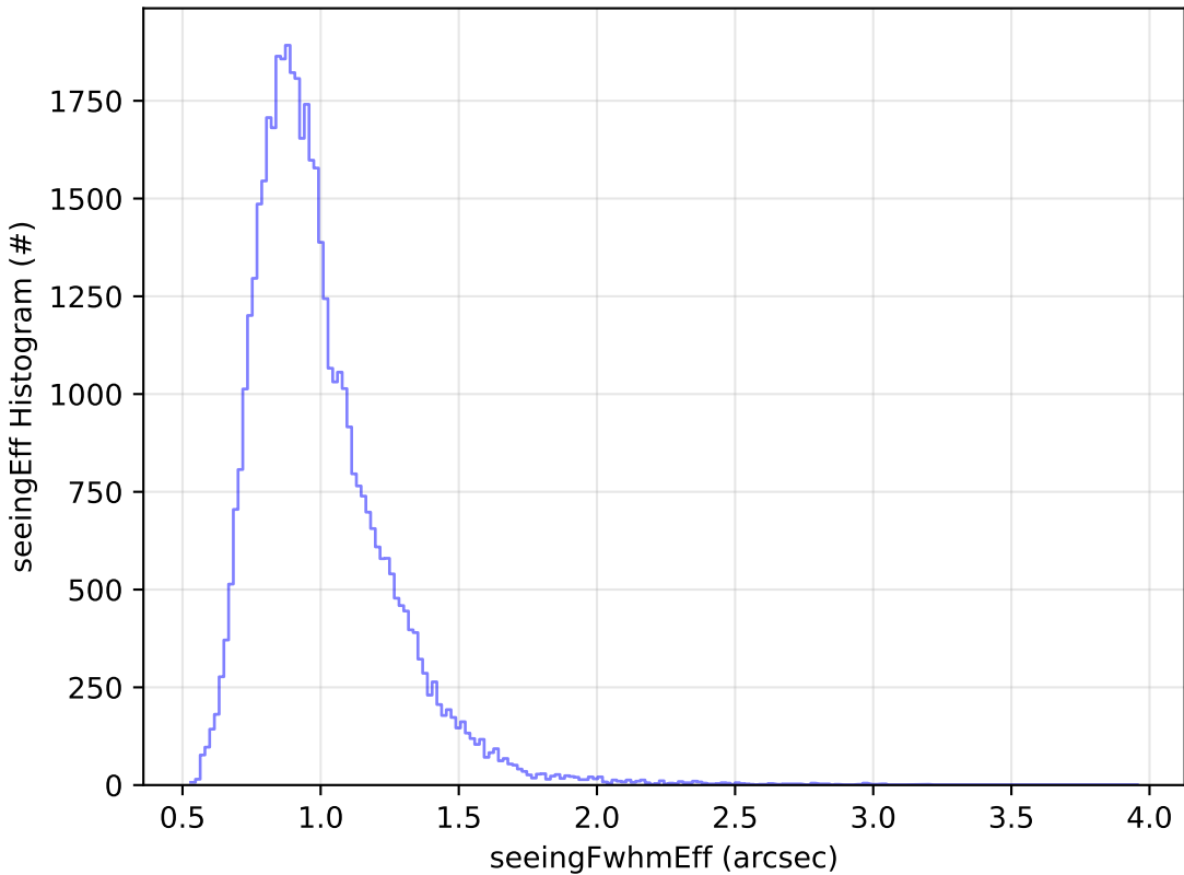
early_u_fpextra2.0_v3.4_10yrs Yr 1 y band: seeingEff Histogram
