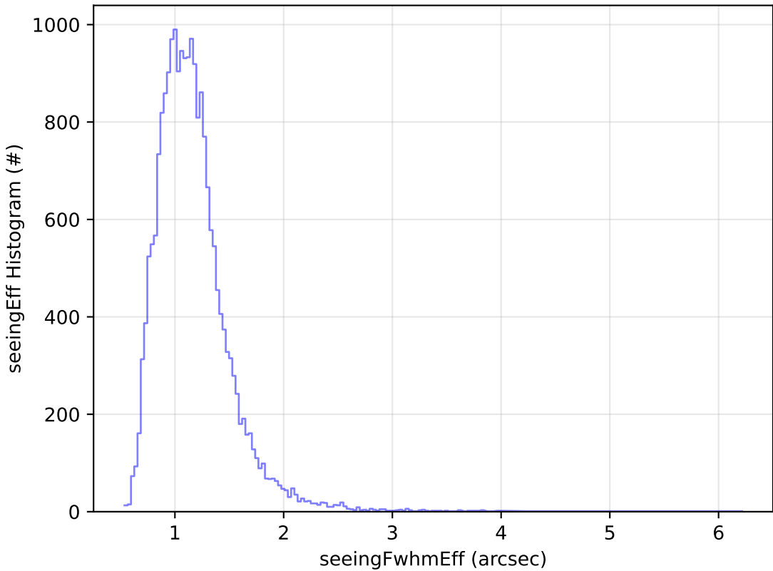
early_u_fpextra2.0_v3.4_10yrs Yr 1 u band: seeingEff Histogram
