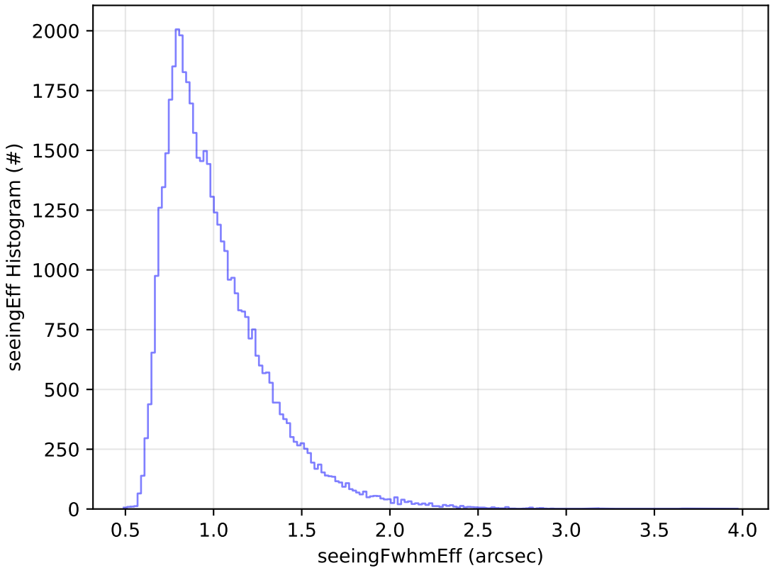
early_u_fpextra2.0_v3.4_10yrs Yr 1 r band: seeingEff Histogram
