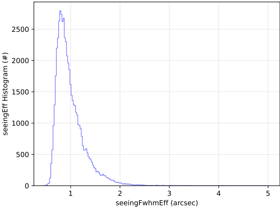
early_u_fpextra2.0_v3.4_10yrs Yr 1 i band: seeingEff Histogram
