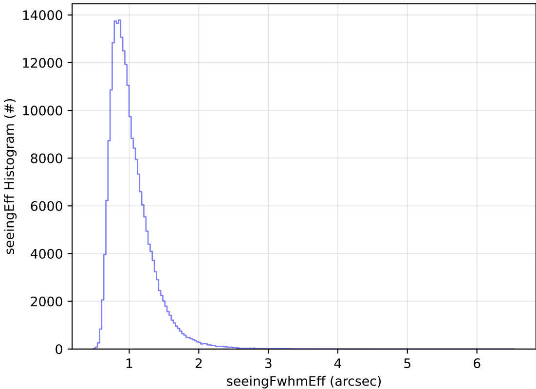
early_u_fpextra2.0_v3.4_10yrs Yr 1 all bands: seeingEff Histogram
