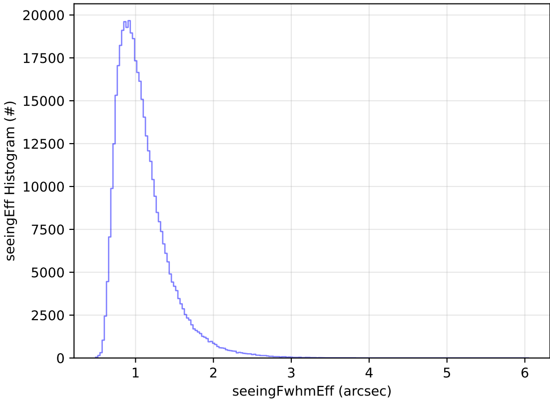
early_u_fpextra2.0_v3.4_10yrs WFD z band: seeingEff Histogram
