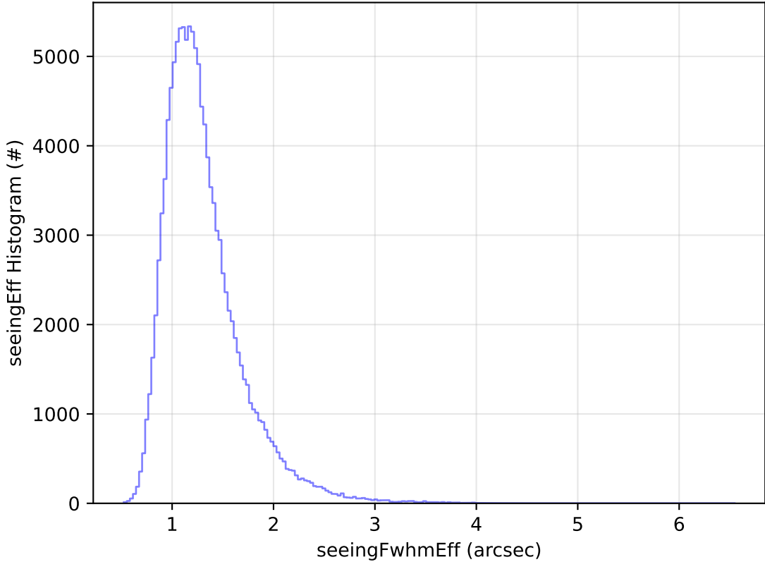
early_u_fpextra2.0_v3.4_10yrs WFD u band: seeingEff Histogram
